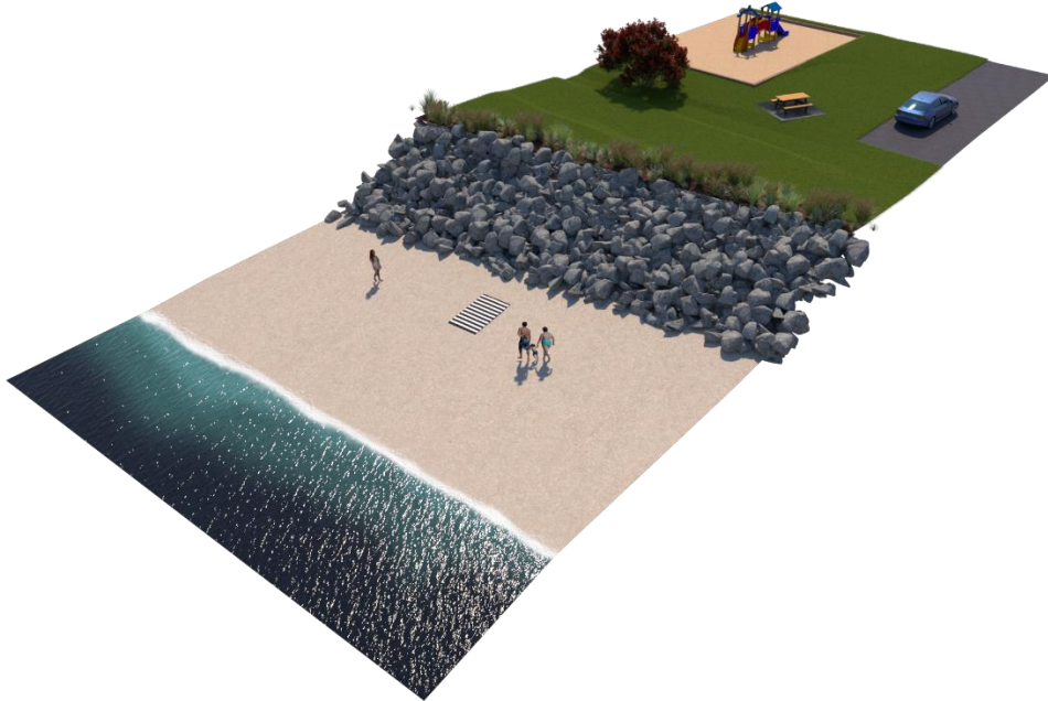
OPTION 1A – HIGH ROCK RIPRAP WALL
