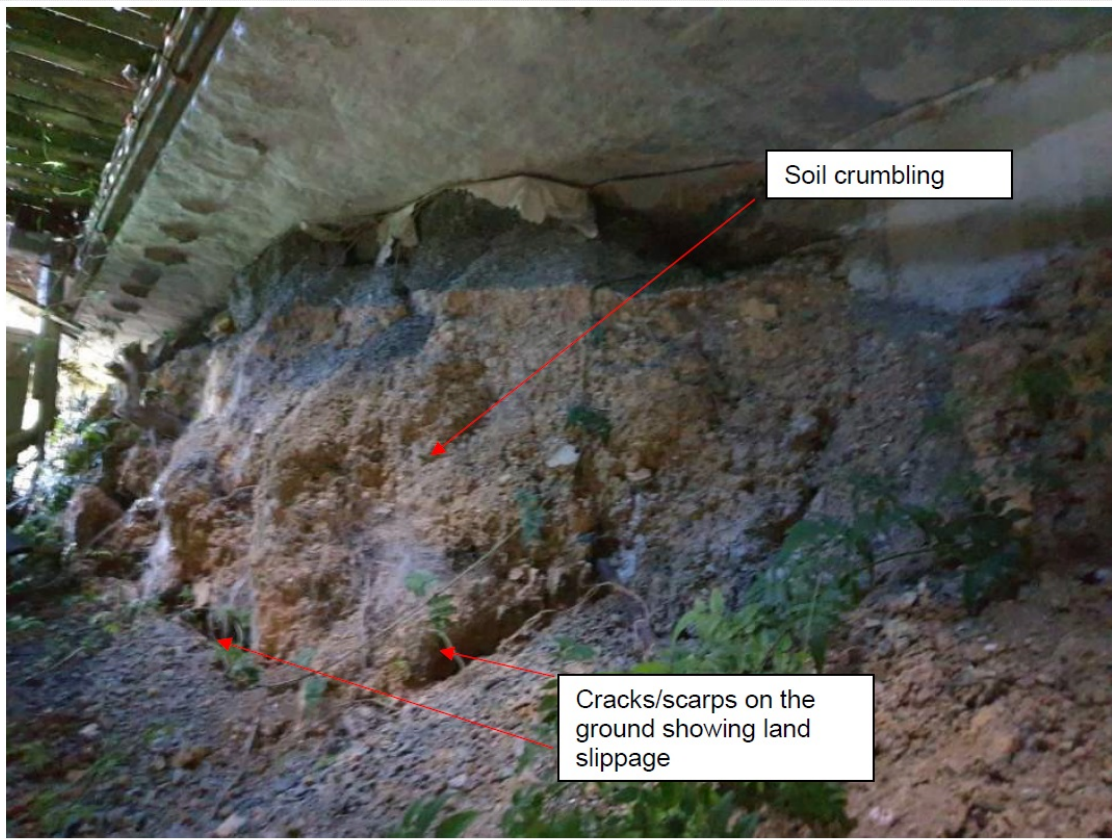
Photo 4: View of the foundation at the southwestern end side of the house. Foundations are getting undermined by the soil fretting – Close Out
