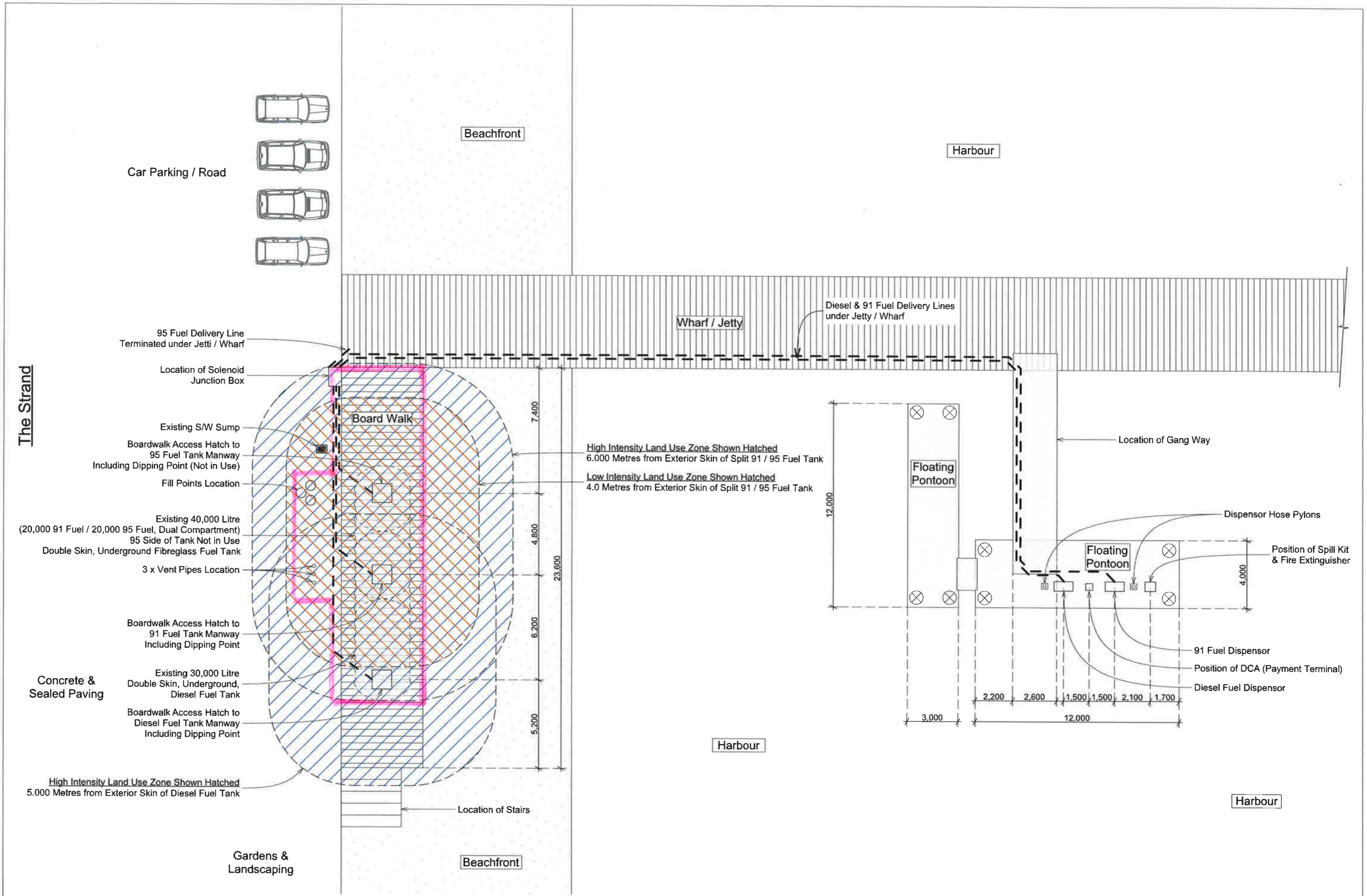
HILU / LILU Compliance Layout
